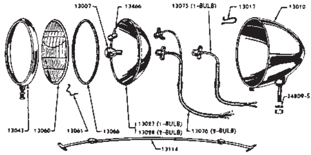
1932 PASSENGER HEADLAMP
