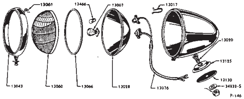
1936 PASSENGER HEADLAMP
